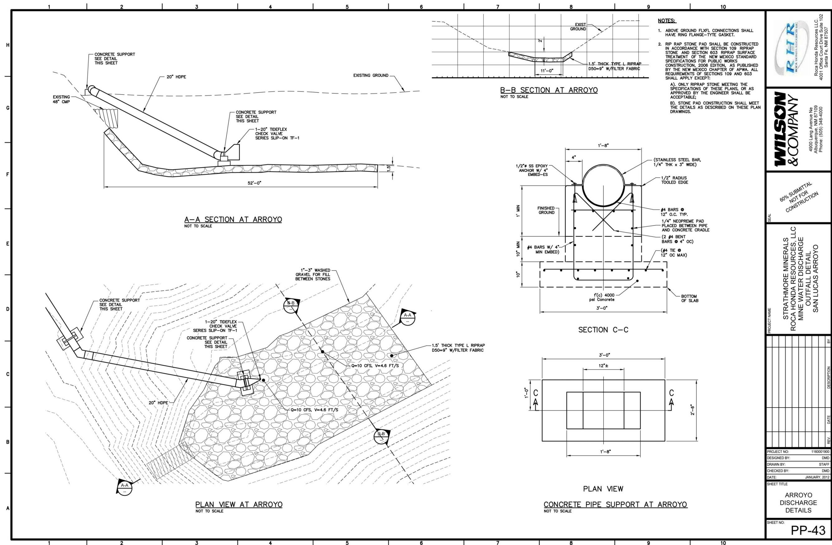
Figure 5-3. Reuse Pipeline Discharge Structure Details
