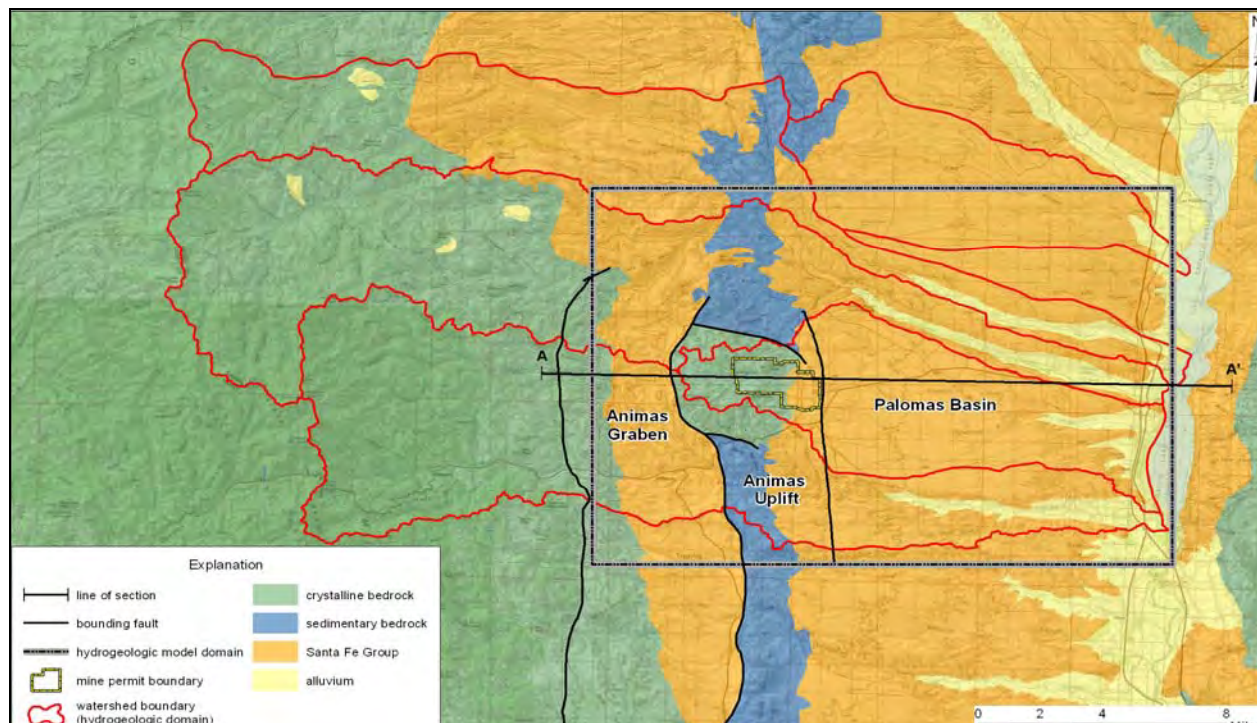
Figure 4.1. Hydrogeologic zones.
