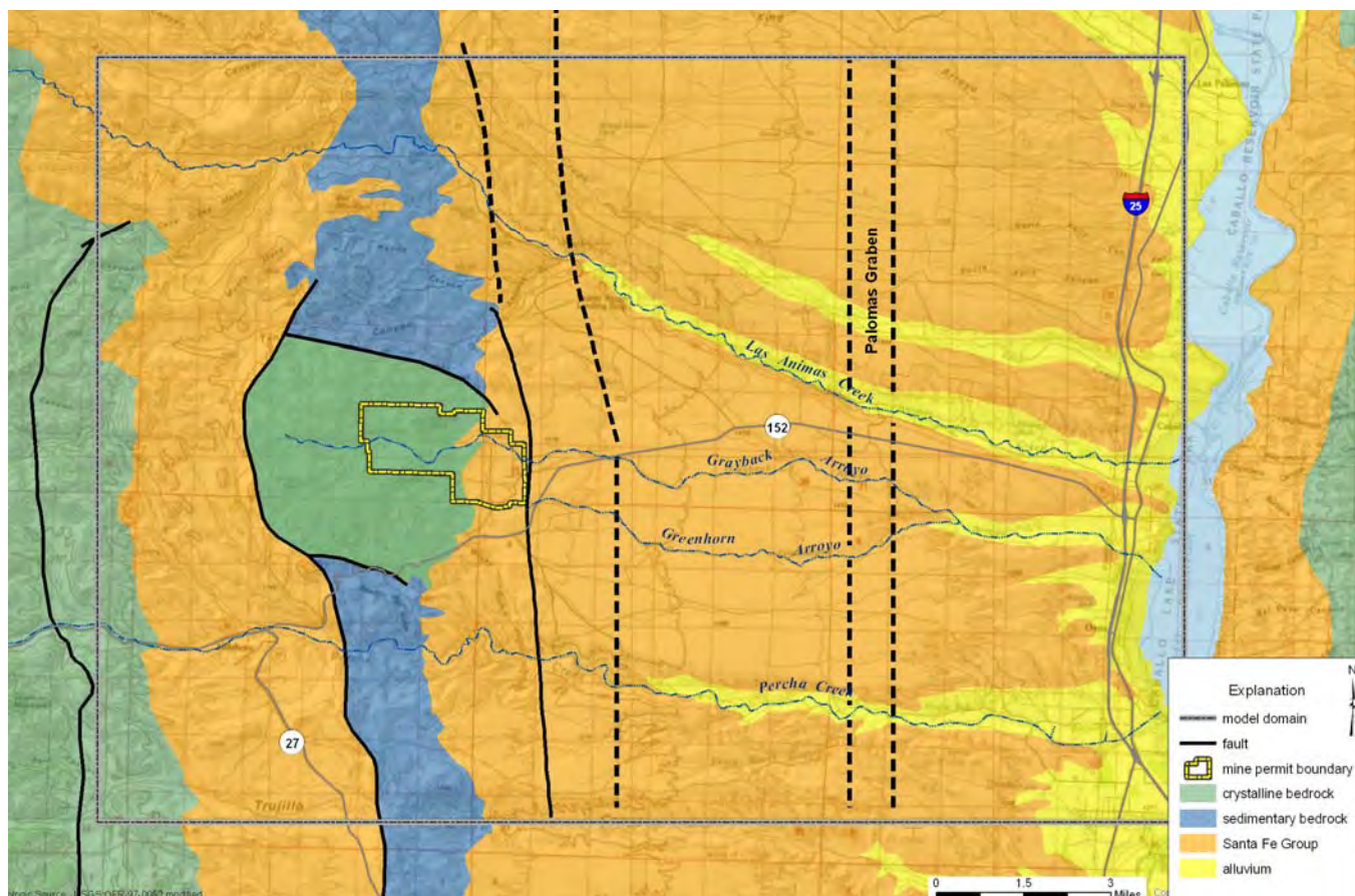
Figure 4.5. Hydrogeologic map of study area.
