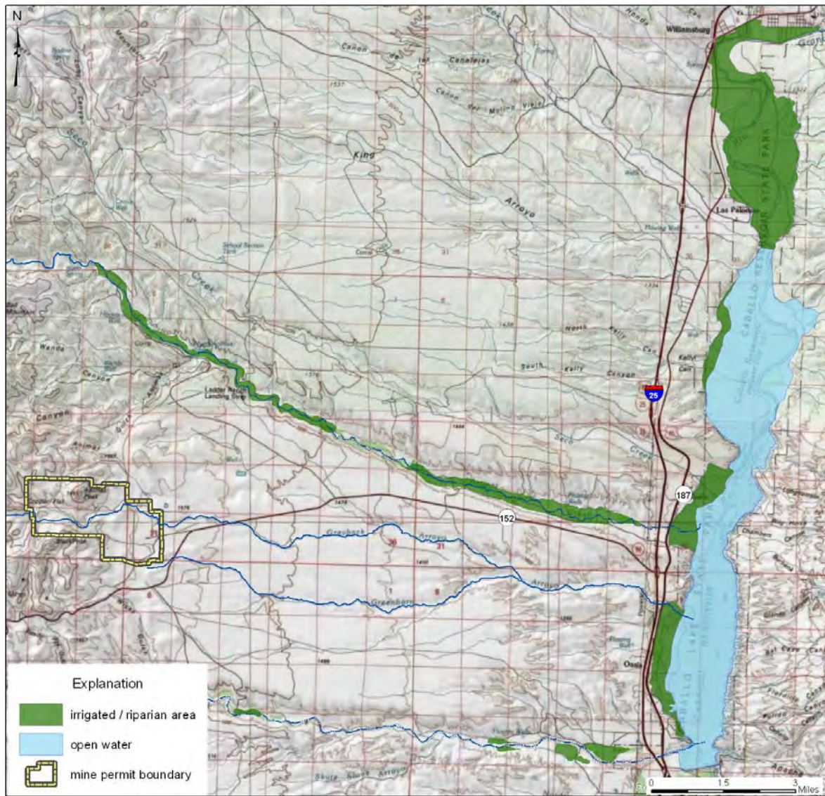
Figure 3.2. Discharge areas.
