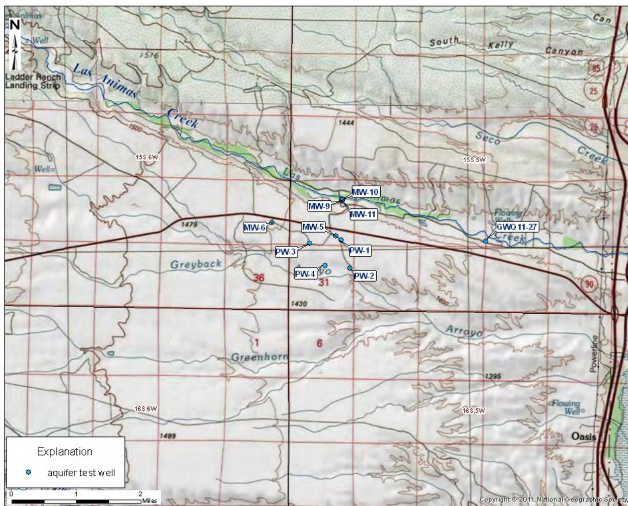
Figure 6.29. 2012 aquifer test pumping and observation locations.
