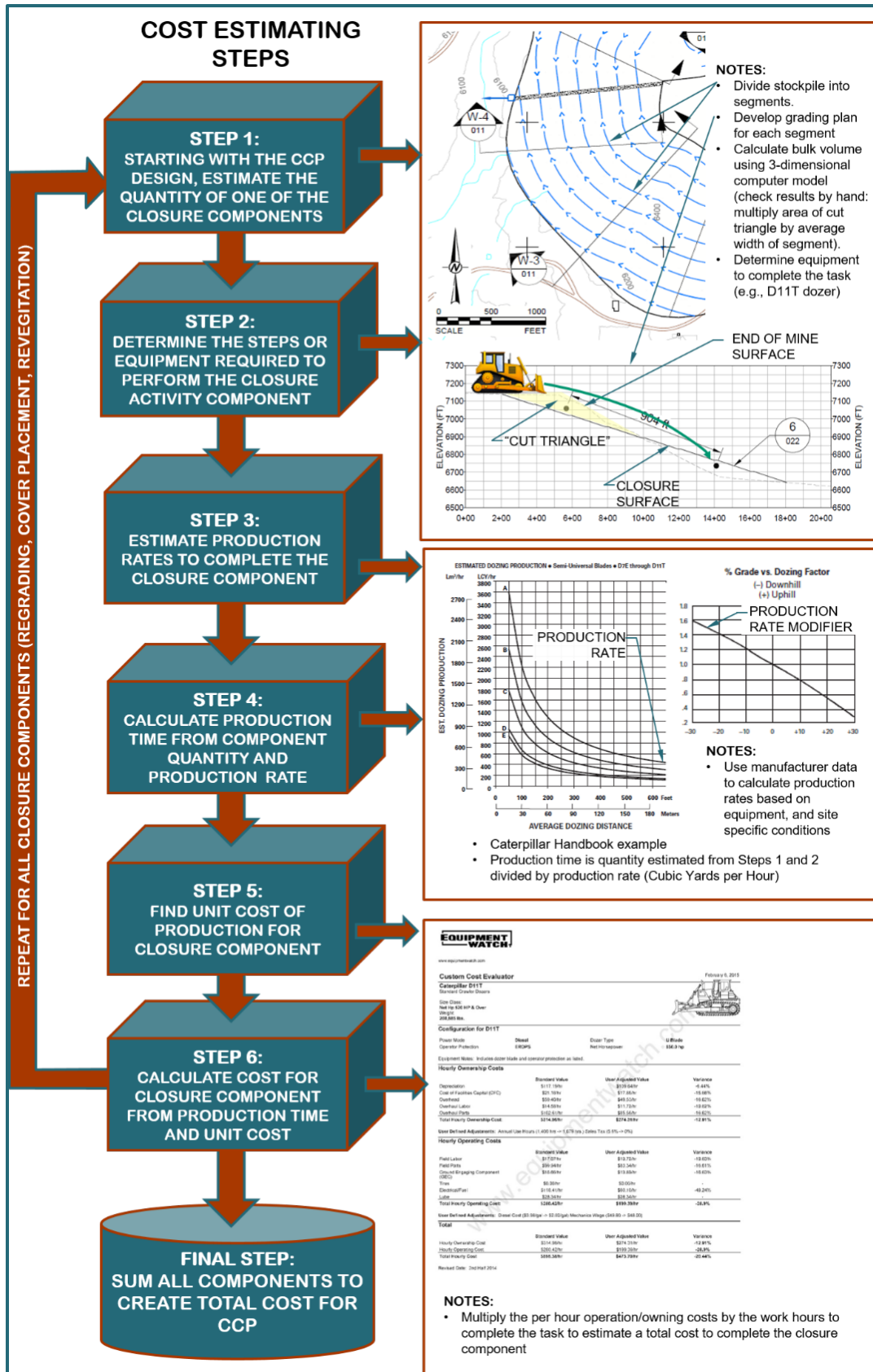
Figure 6 Earthworks Cost Estimating Process
