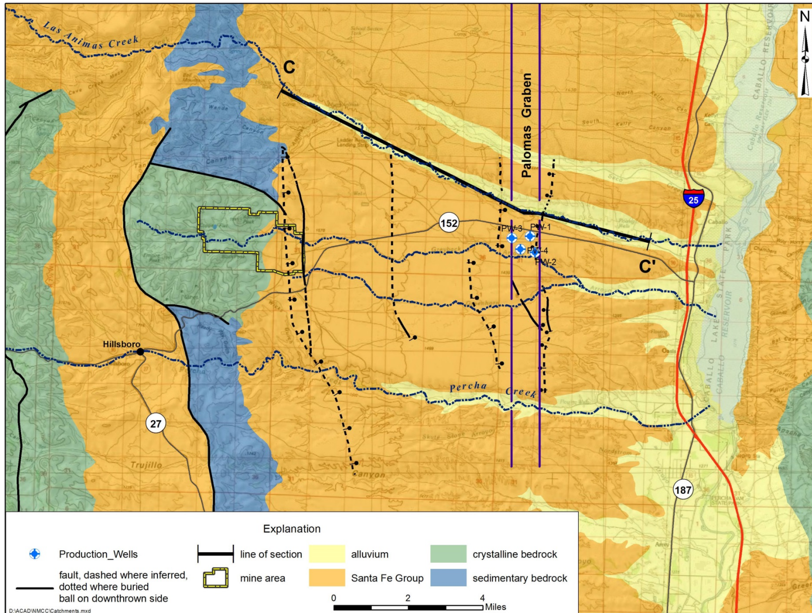
Figure 3.6. Geologic map.
