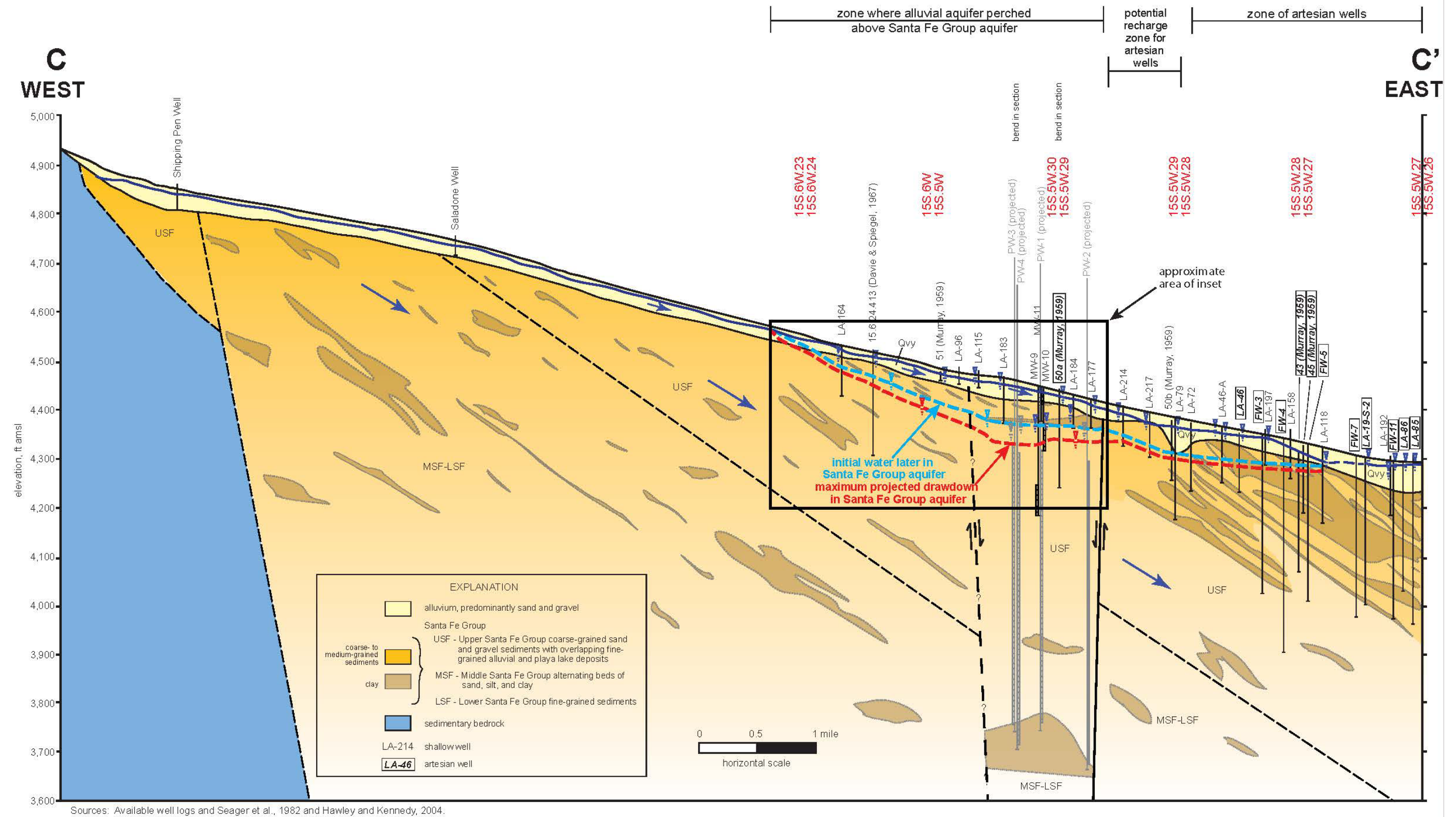
Figure 3.7. Cross-section C-C'.
