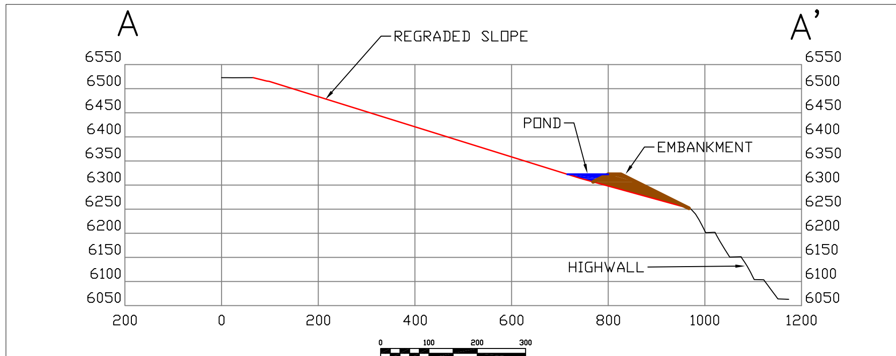
TYRONE MINE Figure 6-Pit Rim Water Management Conceptual Drawing 2C Stockpile Interior Slope
