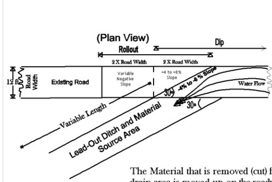
ROLLING DIP
