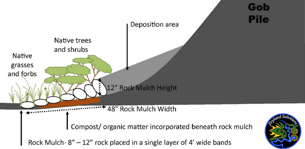
GOB TOE TREATMENT
