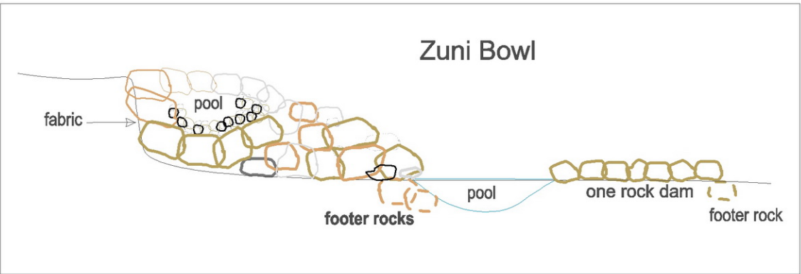
ZUNI BOWL
