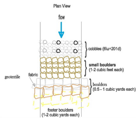
DROP STRUCTURE
