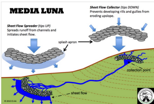
MEDIA LUNA
