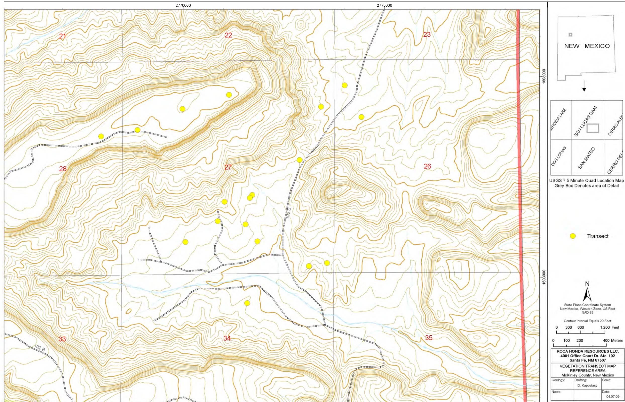
Figure 4-3. Transect Line Locations in the Reference Area (T14N, R8W)
