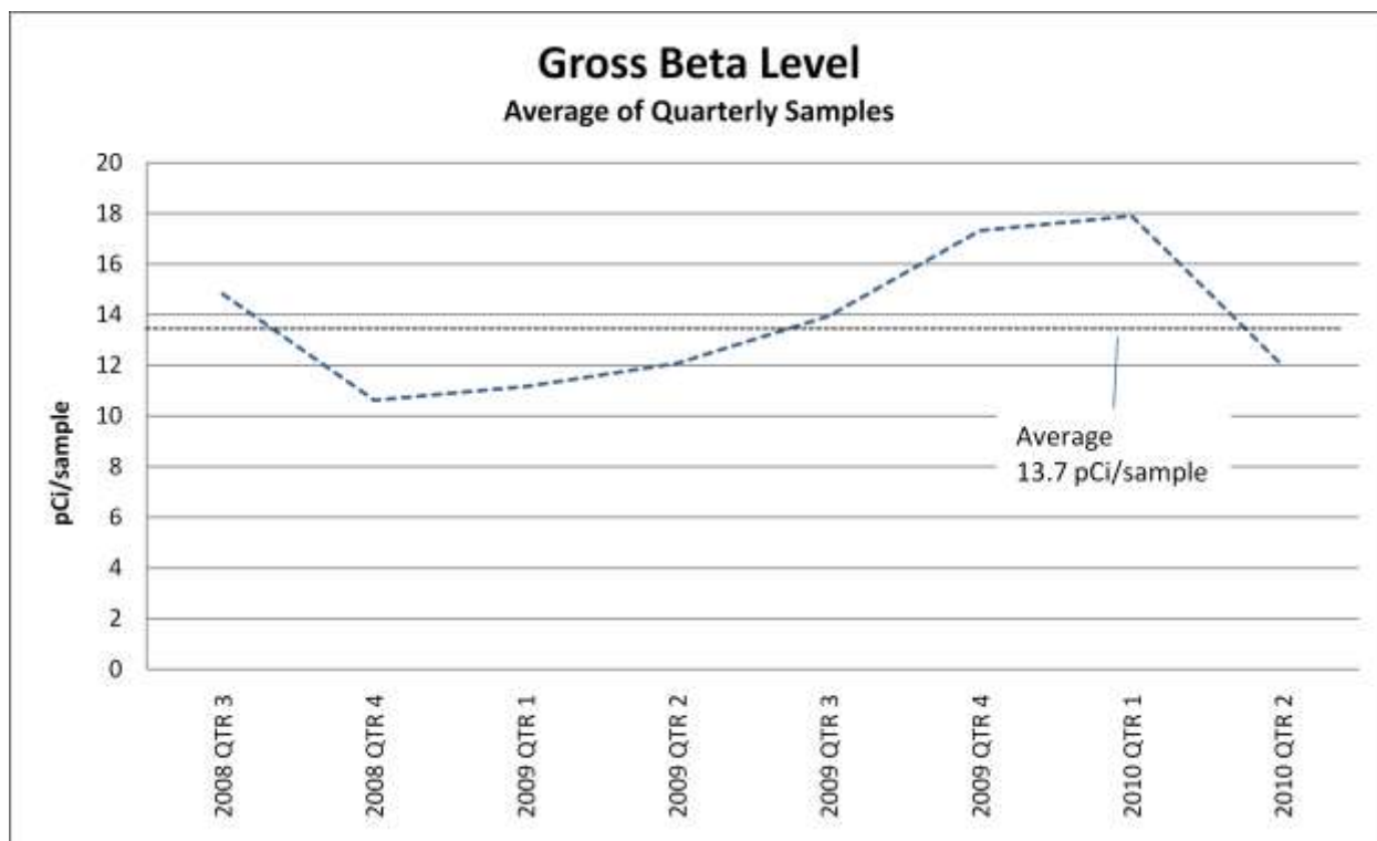
Figure 2-8. Gross Beta Air Filter Sampling (Source: Table 2-4)
