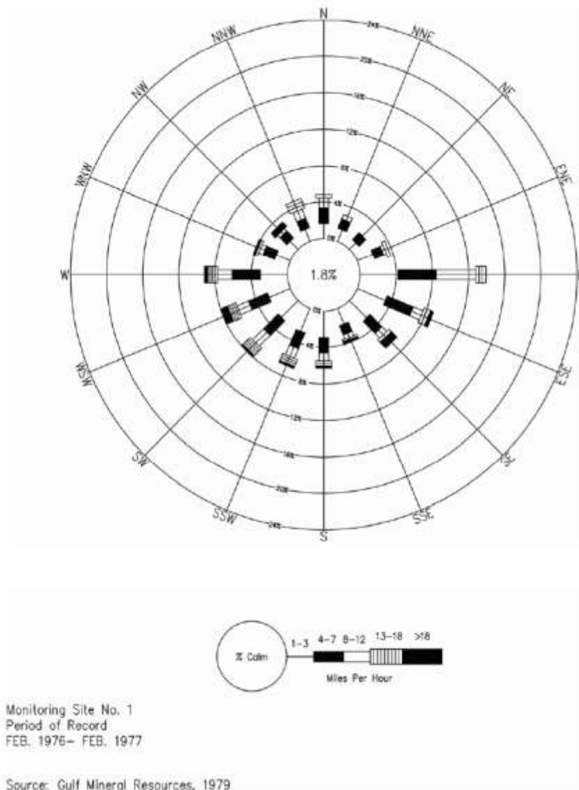
Figure 2-2. Wind Rose Diagram for GMRC Monitoring Site
