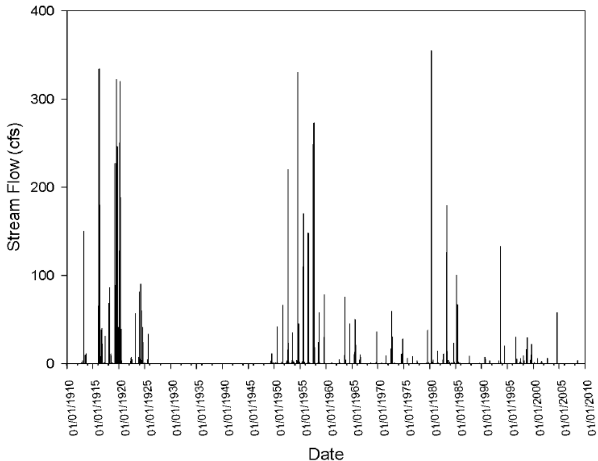
Figure 8-5. Daily Stream Flow from Rio San Jose at Grants (USGS Gaging Station 8343000)
