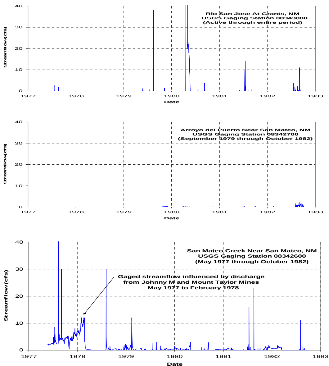
Figure 8-3. Mean Daily Stream Flow for San Mateo Creek, Arroyo del Puerto, and Rio San Jose 1977 through 1982
