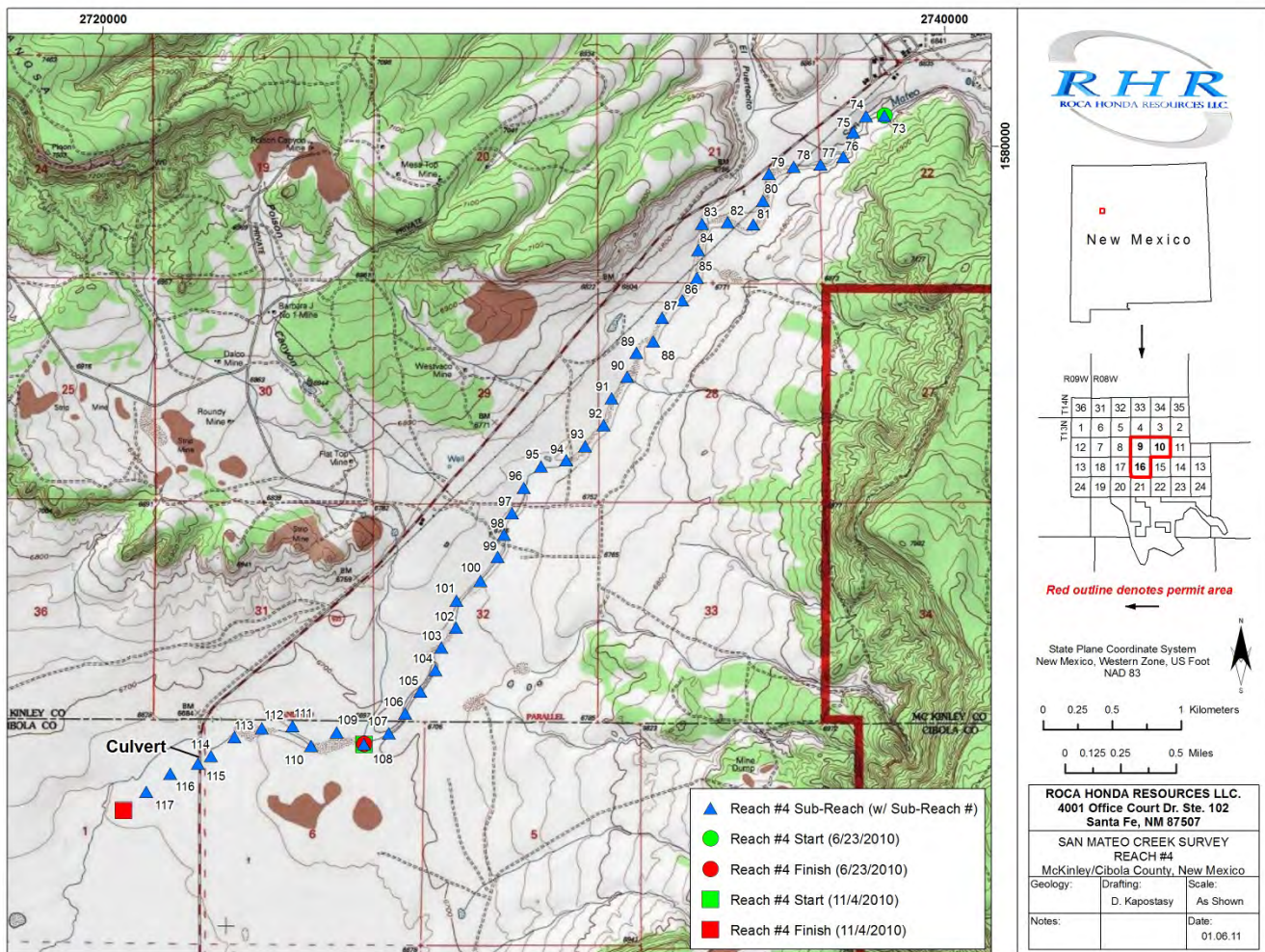
Figure 4. Location of Reach #4 Sub-reaches
