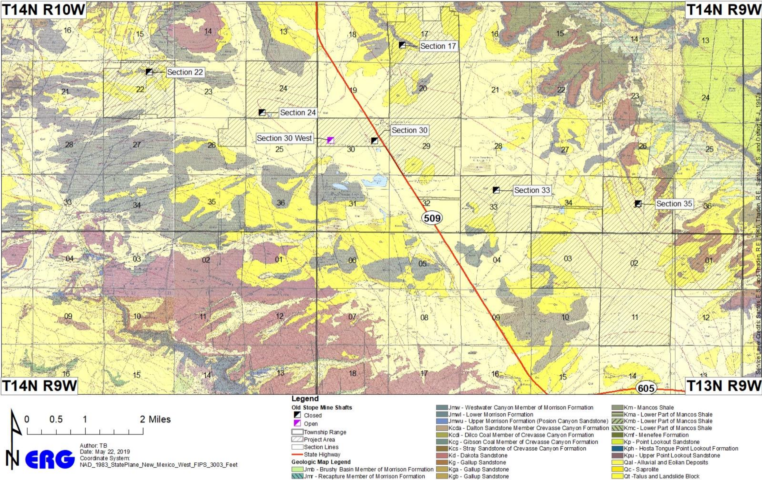
Figure 9. Geologic map of the Ambrosia Lake Valley Note: Geologic map is from Santos and Thaden (1966); Thaden, Santos, and Ostling (1967).
