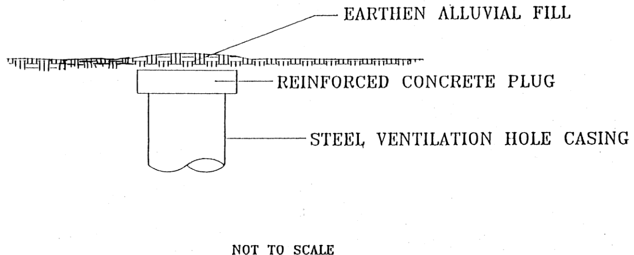
Figure 13 Schematic of capping process for closure of ventilation holes.
