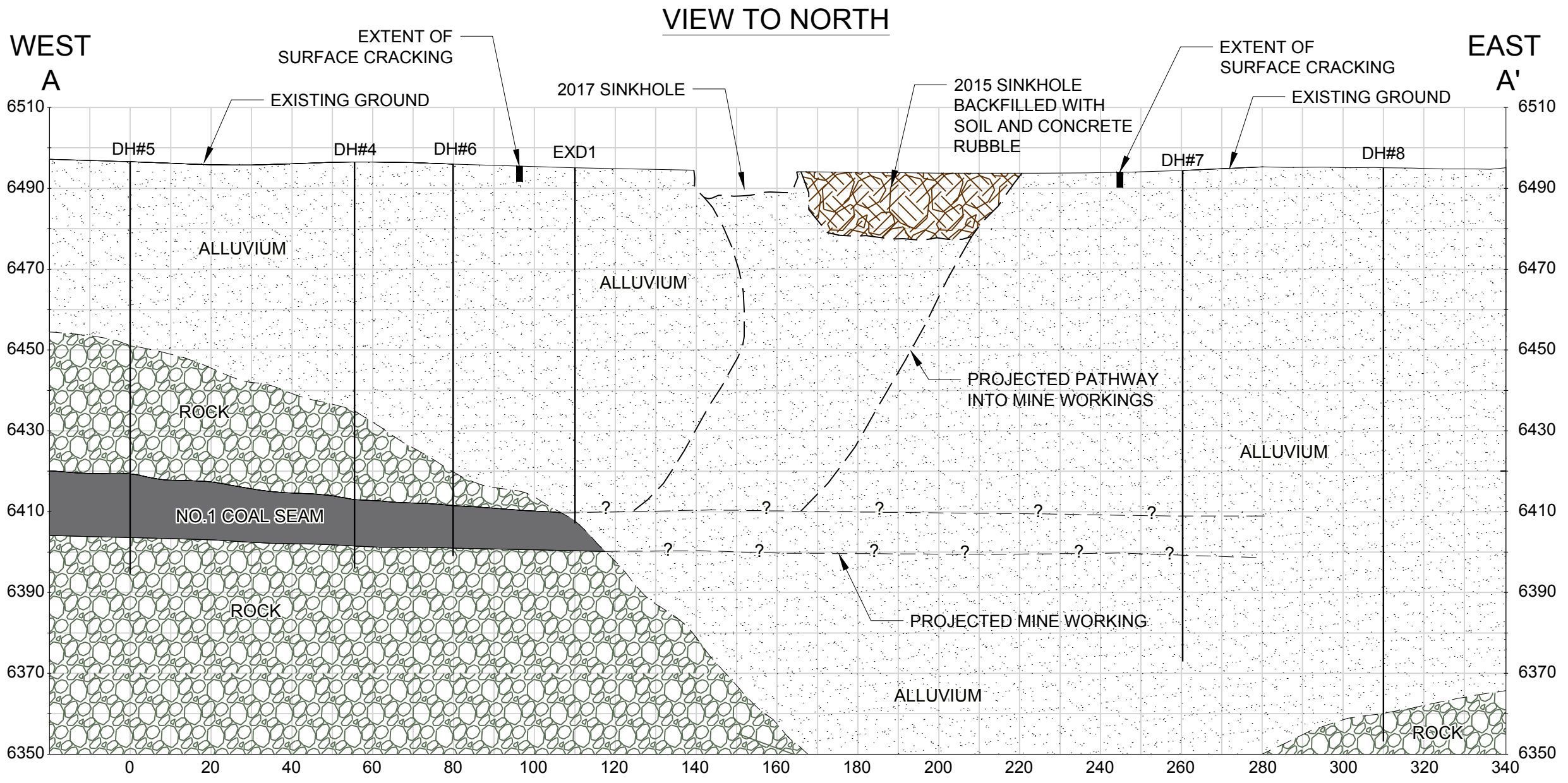
SCALE 1"=30' A CROSS SECTION LOOKING NORTH 1
